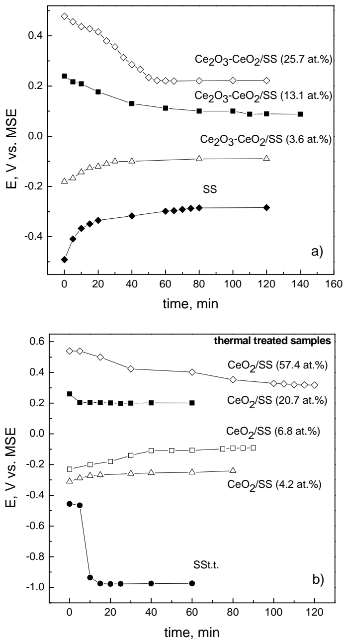
Fig. 4. Open circuit potential vs. time curves for SS (a) and SS t.t. (b), as well as for the systems CeO 2 -Ce 2 O 3 /SS (a) and CeO 2 -Ce 2 O 3 /SS t.t. (b), containing different concentrations of Ce, obtained in 0.1 N H 2 SO 4 .
