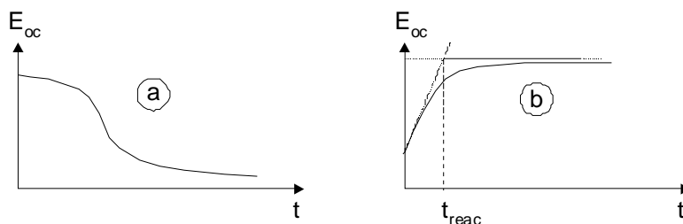
Fig. 7. Schematic representation of the evolution of E_{oc} with immersion time in the case of (a) corrosion, and (b) passivation. The graphical determination of t_{reac} in the case of passivation is shown in (b).
