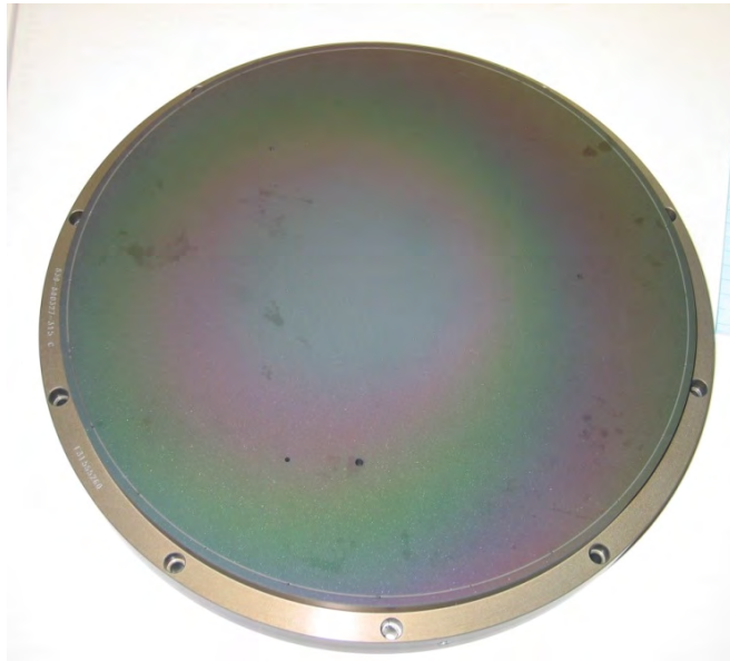
Fig. 7. A uniform AIOF film (rainbow color) covers the ceramic surface of a used electrostatic chuck after silicon etch processes.
