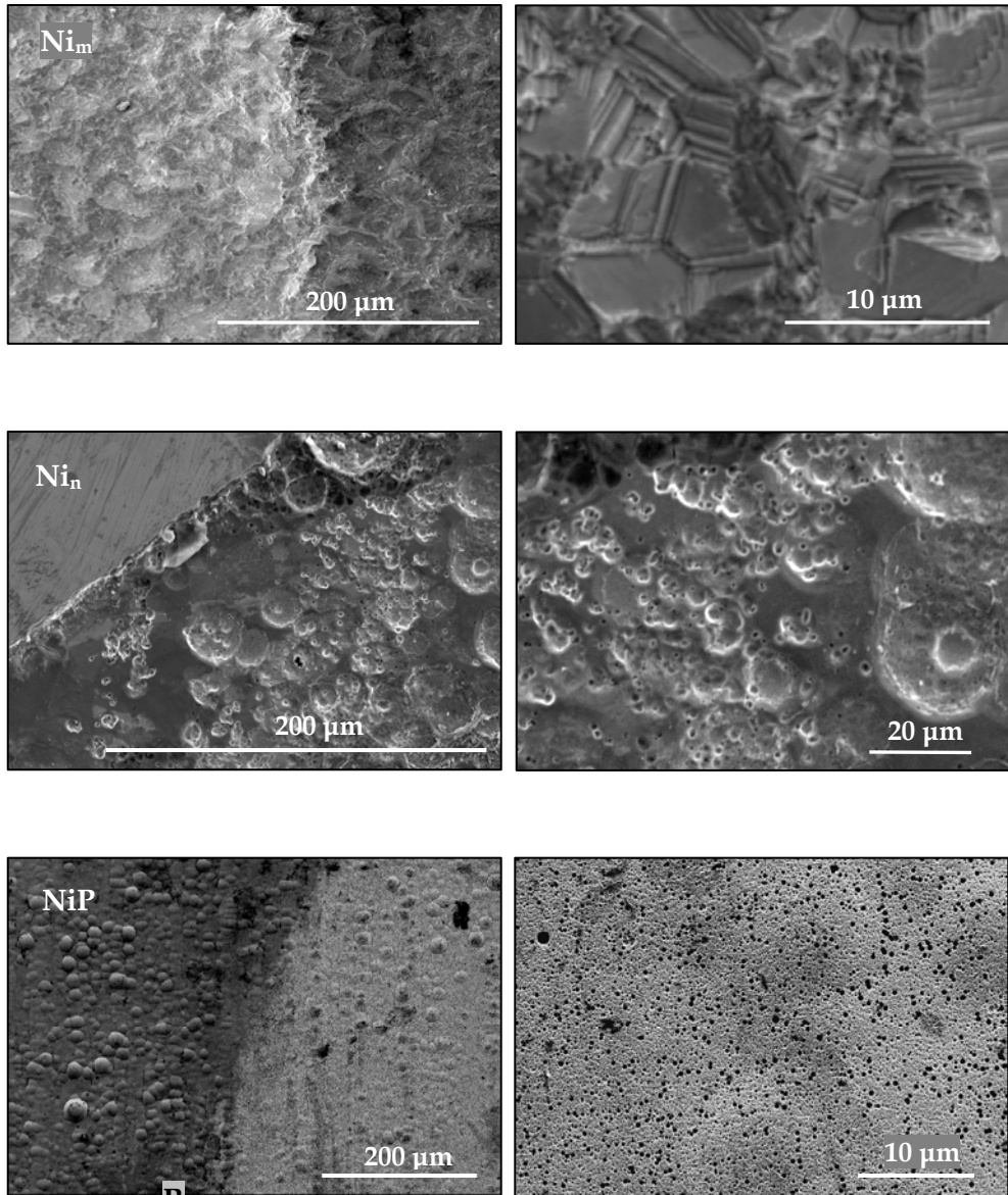
Fig. 24. SEM images of the surface of Ni_m , Ni_n and NiP alloy after corrosion tests in an environment of 0.5M NaCl solution.
