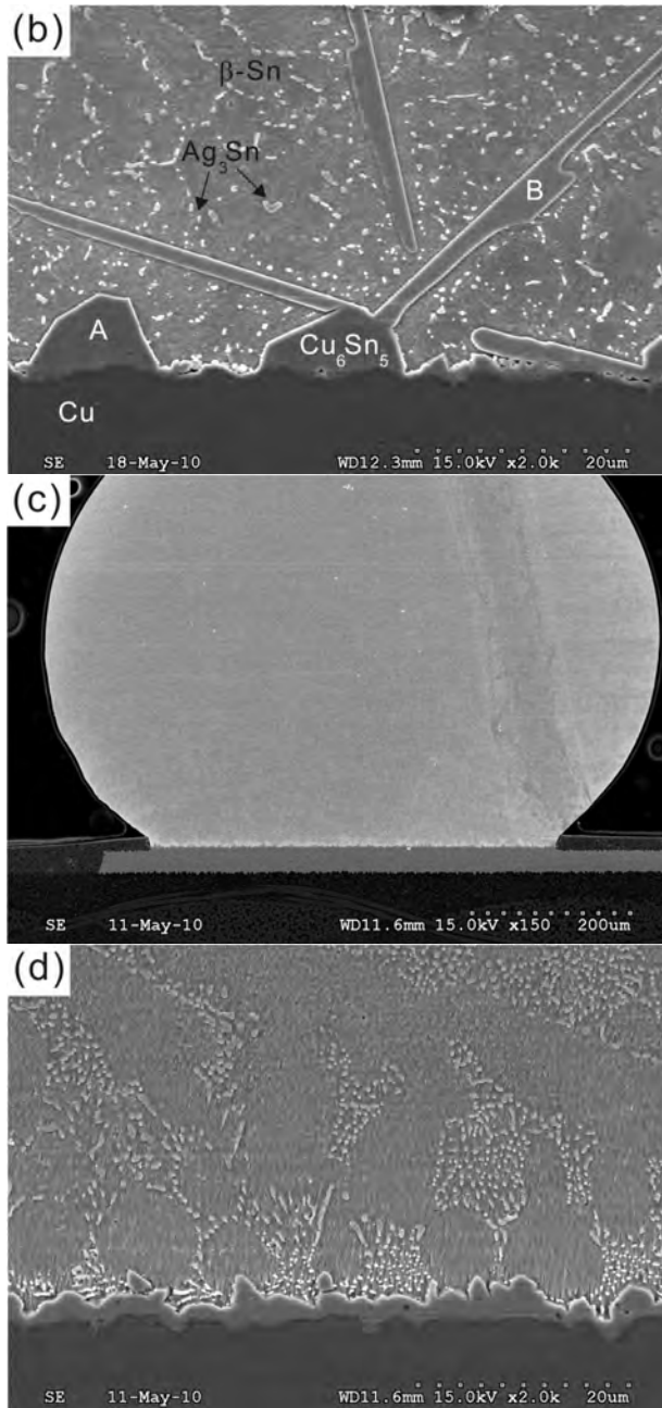
Fig. 12. Morphology of intermetallic compounds formed at the interfaces of the as-reflowed solder joints: (a) Sn3.5Ag0.5Cu, (b) (a) magnifications ; (c) d Sn3.5Ag0.5Cu-0.75TiO 2 ; (d) (c) magnifications [58].
