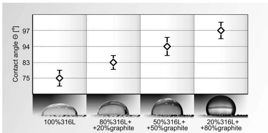
Fig. 13. Contact angle evaluated for graphite-steel composites.
