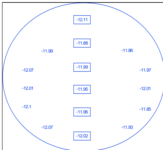
Fig. 14. The leakage current of gate oxide in log scale indicates that there is no damage to gate oxide when a boron carbide coated chamber is used.
