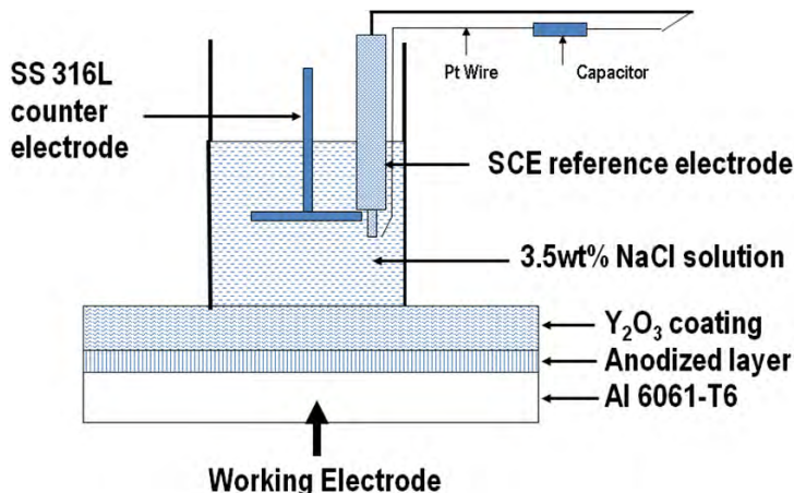
Fig. 27. Electrochemical cell configuration during EIS study of Y_2O_3 coated anodized aluminum in 3.5wt% NaCl solution [78].
