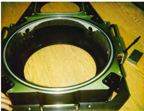
Fig. 5. Anodized aluminum is fully removed under Cl_2/BCl_3 plasma after only 1,800 wafers in production (about 60 RF hours). The special attacking pattern depends on the local plasma density and gas concentration.
