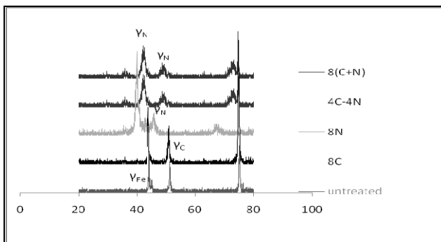
Fig. 10. Comparison of XRD patterns of treated specimens.
