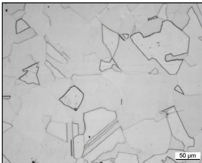
Fig. 4. Microstructure of a uniform and solution annealed austenite with \sim 0,6\% N.
