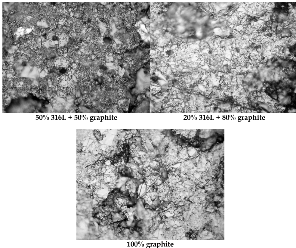
Fig. 9. Microstructures of graphite-steel composites, magnitude 100 x.
