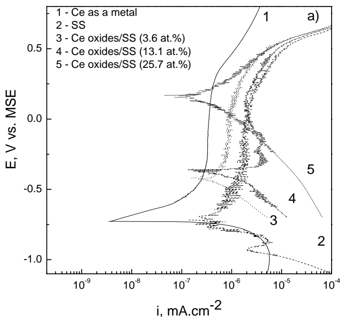
Fig. 3a. Potentiodynamic E - \lg i curves for Ce (1), for SS (2) and for the systems CeO_2 - Ce_2O_3 /SS containing different concentrations of Ce (3-5), obtained in 0.1 N H_2SO_4 .
