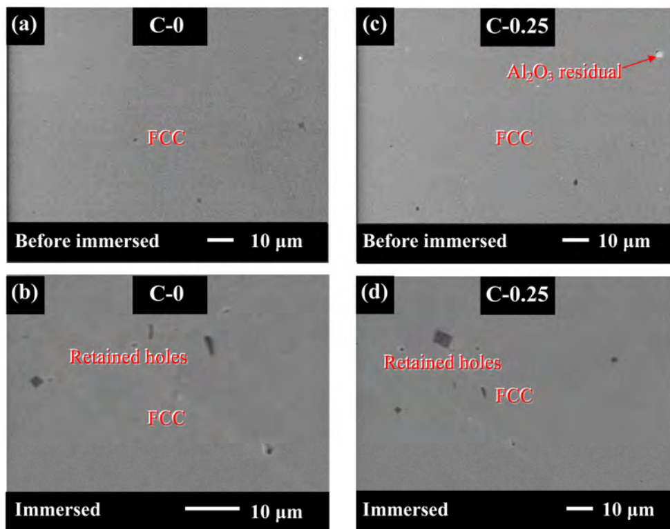
Fig. 11. Metallograph of alloys C-0 ((a) & (b)) and C-0.25 ((c) & (d)). (a) & (c), before; and (b) & (d), after immersion. Retained holes were from cast procedure, and Al_2O_3 residuals were from polishing procedure.
