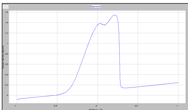
Fig. 15. Cyclic voltammogram of electrodes coated with paint.
